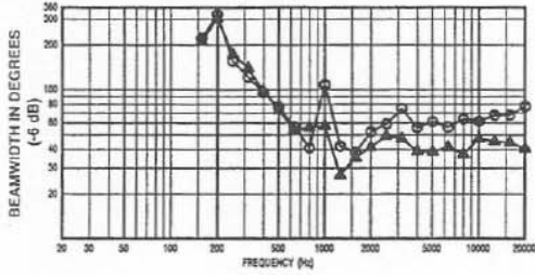
FIGURE 2 — Beamwidth vs. Frequency
